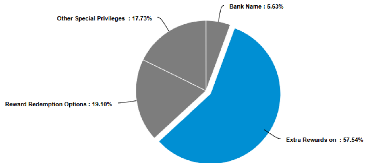
Attribute Importance
